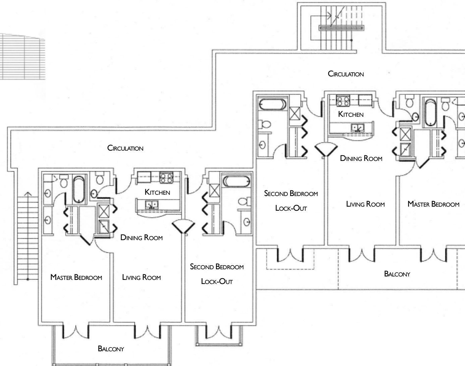
TYPICAL TWO-BEDROOM LOCKOUT UNIT FLOOR PLAN
